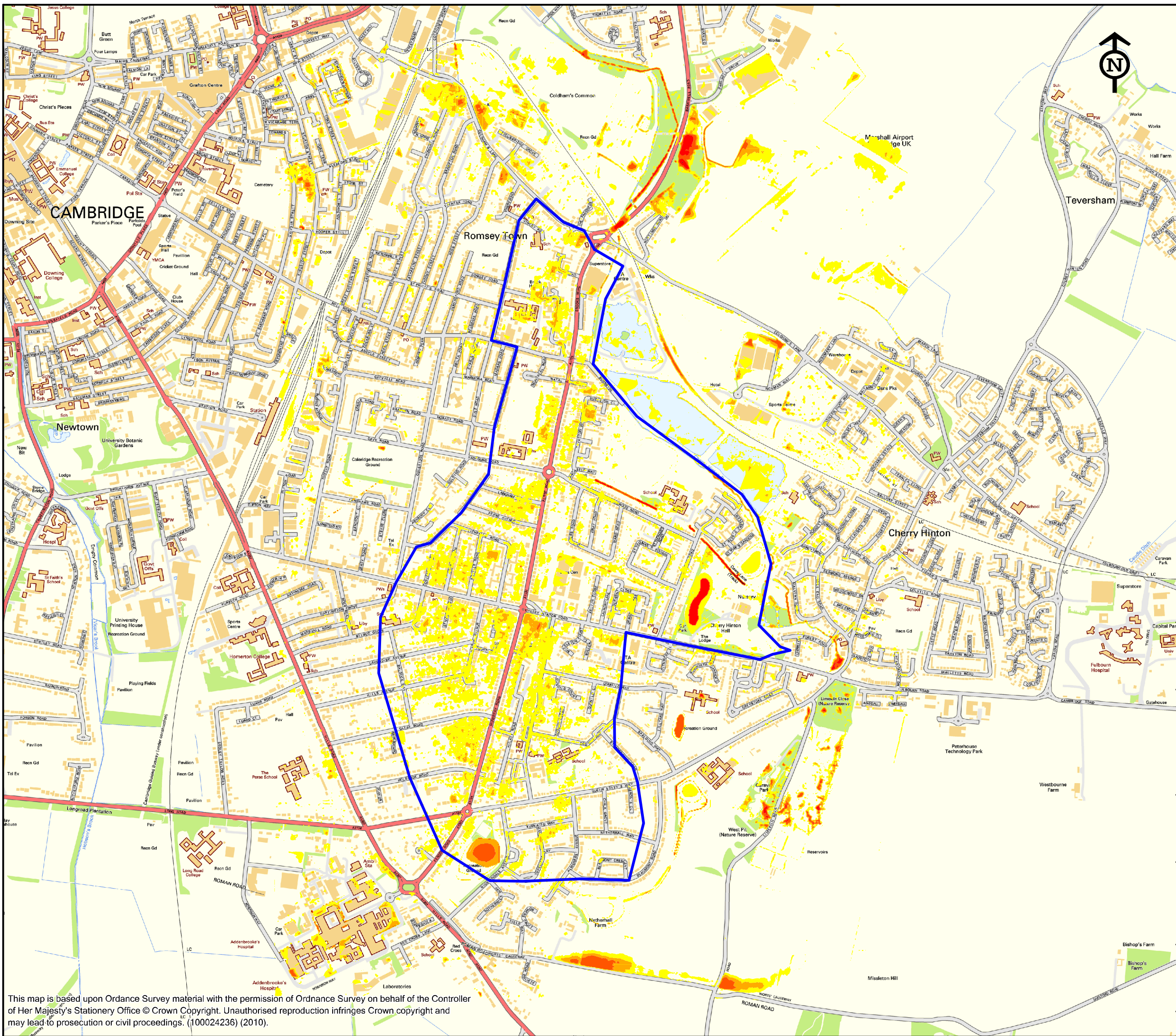
FIGURE G7 0.5% AEP "OPTION C1" PLUVIAL MODELLING MAXIMUM DEPTH CHERRY HINTON
